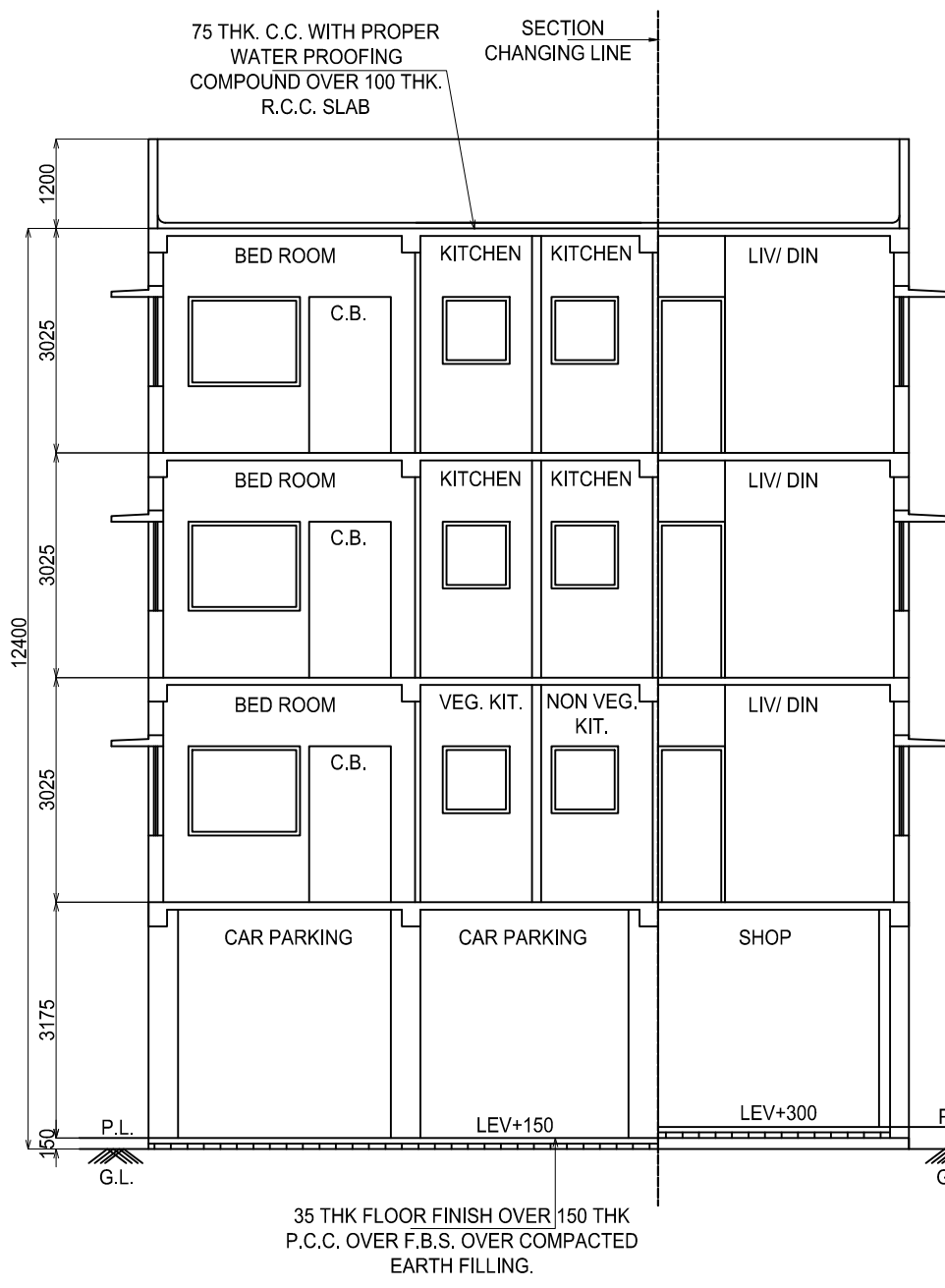
SECTION-BB
