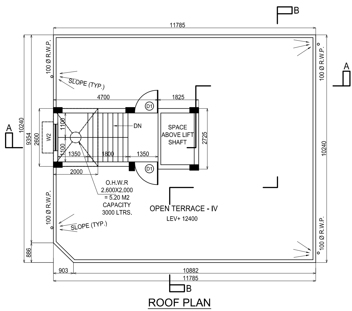
ROOF PLAN
