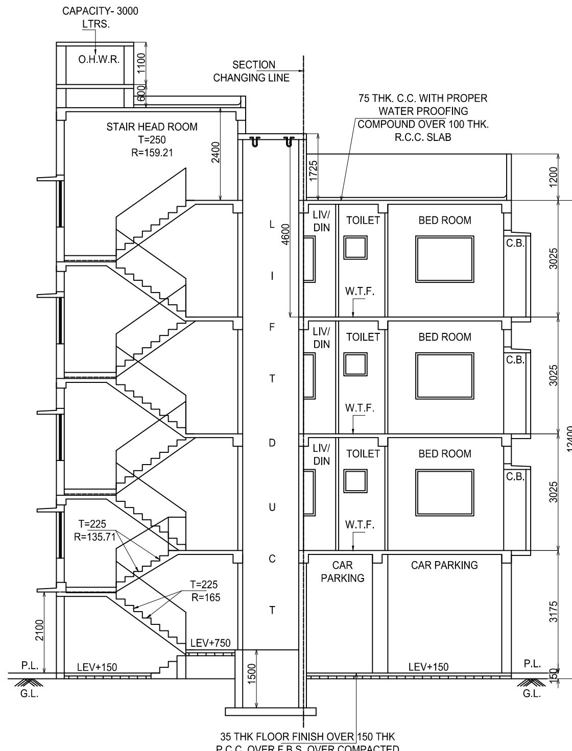
SECTION-AA
